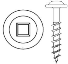
Drawer Front Screw Recex #8 x 1-1/4 M-R20-3102
